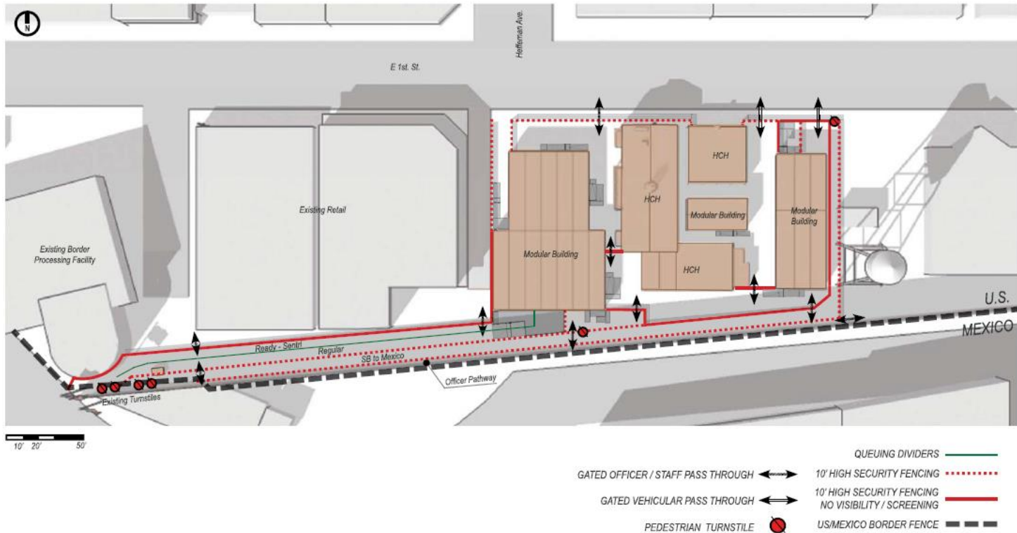
SECURITY FENCE DIAGRAM
